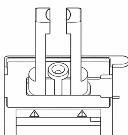
Figure 7 – 20 ml magnetization accessory assembly
